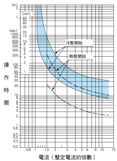
●TH-T65SR、T65KPSR ●TH-T100SR、T100KPSR
