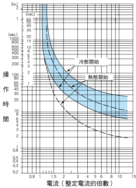
●TH-T50SR、T50KPSR
