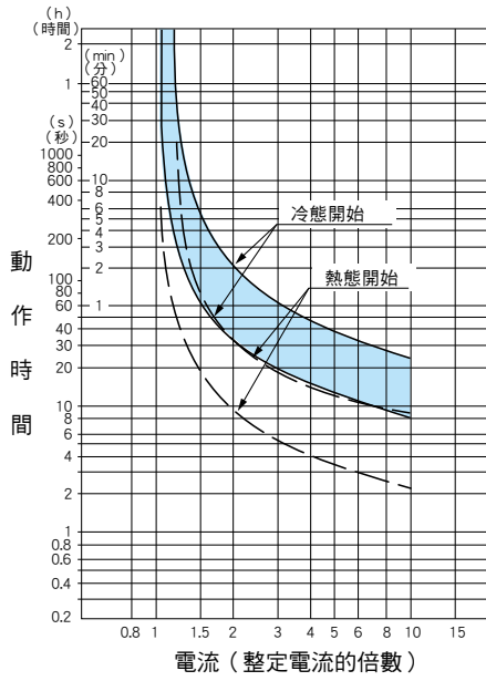
●TH-T18SR
