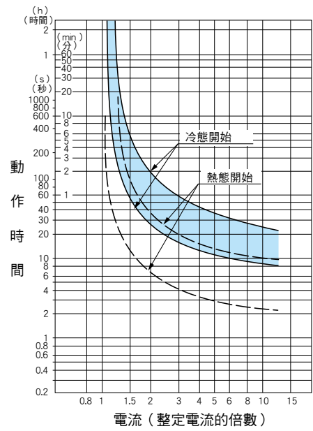
●TH-T65SR、T65KPSR ●TH-T100SR、T100KPSR
