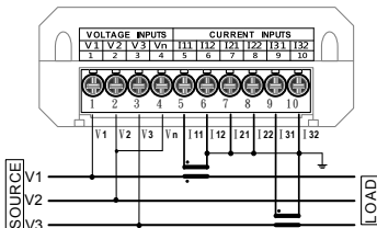
3P3W-電壓直入無PT/2CT [設定:3P3W2CT]
