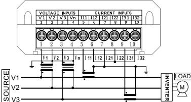
3P3W平衡負載-2PT/1CT [設定:3P3W1CT]
