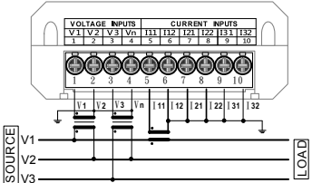
3P3W平衡負載-2PT/1CT [設定:3P3W1CT]
