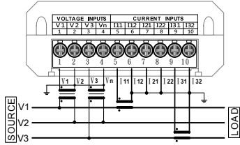
3P3W-2PT/2CT [設定:3P3W2CT]
