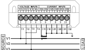
3P3W平衡負載-電壓直入無PT/1CT [設定:3P3W1CT]
