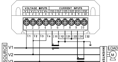
3P3W平衡負載-電壓直入無PT/1CT [設定:3P3W1CT]
