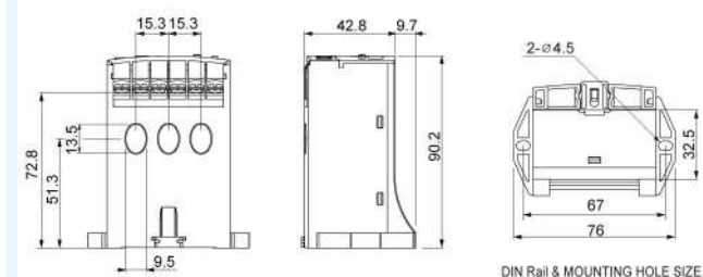
EOCR-SE2
