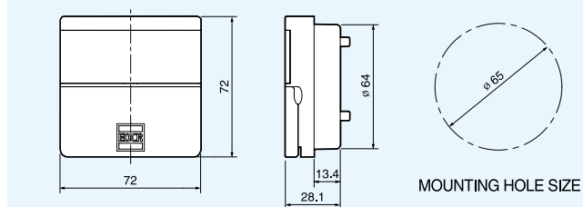
EOCR-PDM (Display)
