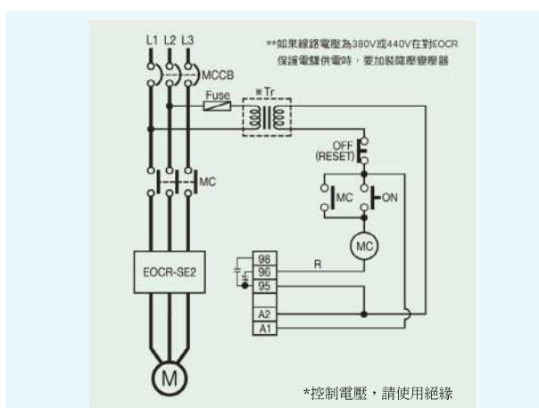
EOCR-SE2
