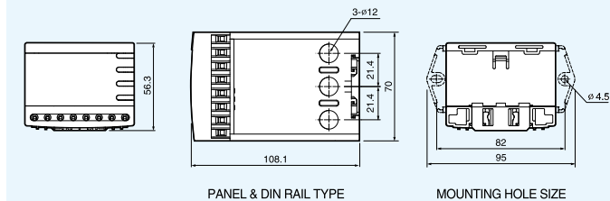
EOCR-3DM2-HZ(過孔式)
