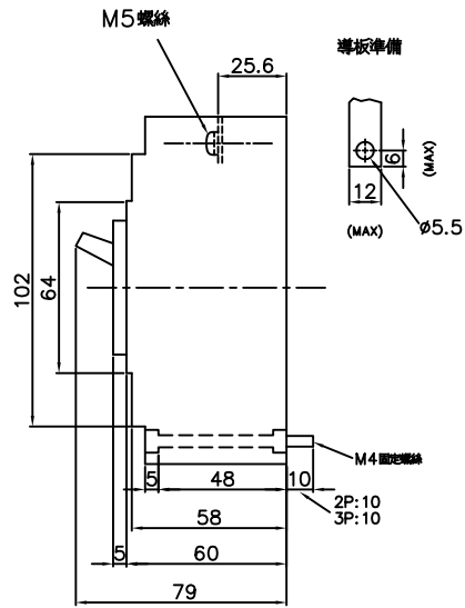
TO-50E, TO-50EC
