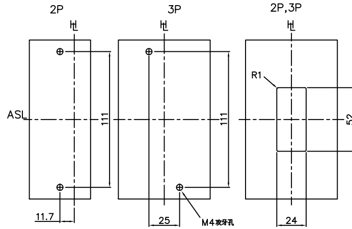
TO-50E TO-50EC
